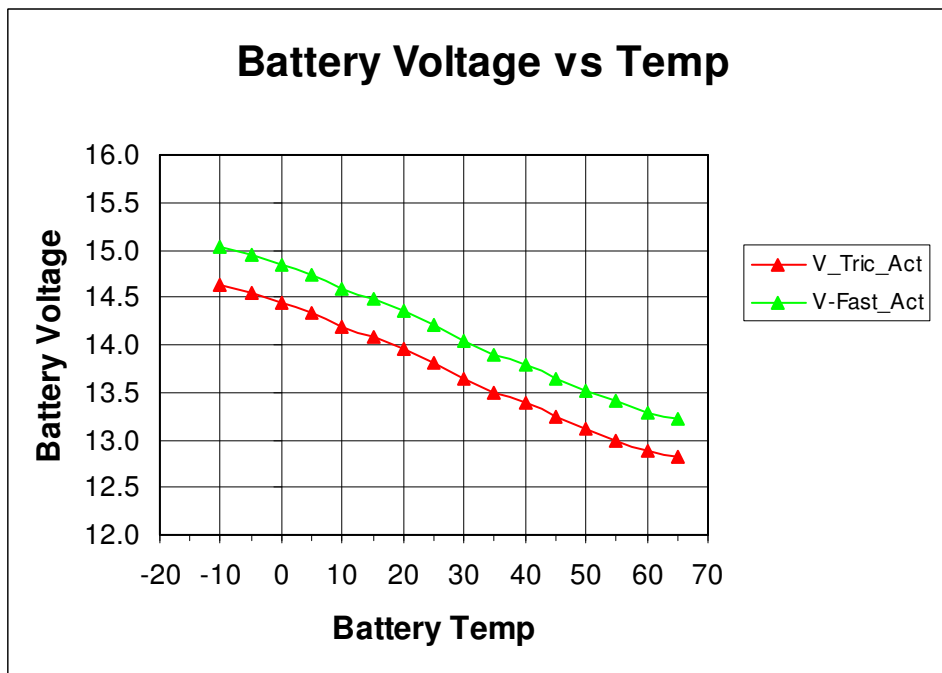
Battery voltage versus temperature during fast a & trickle charge
